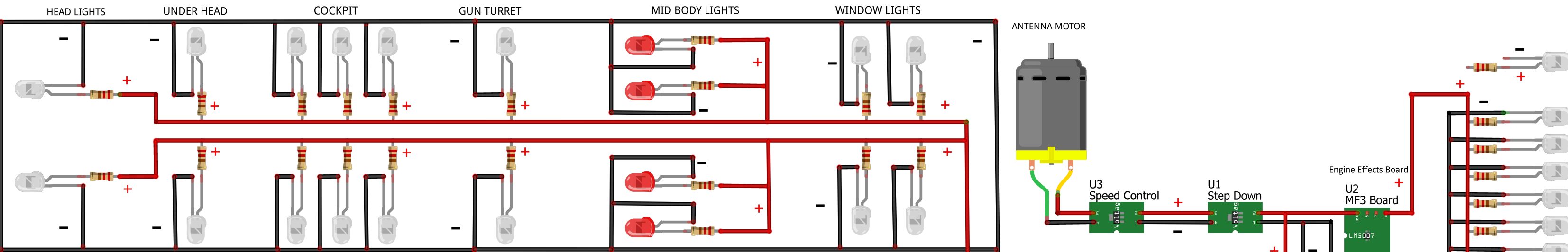
BLOCKADE RUNNER WIRING DIAGRAM
