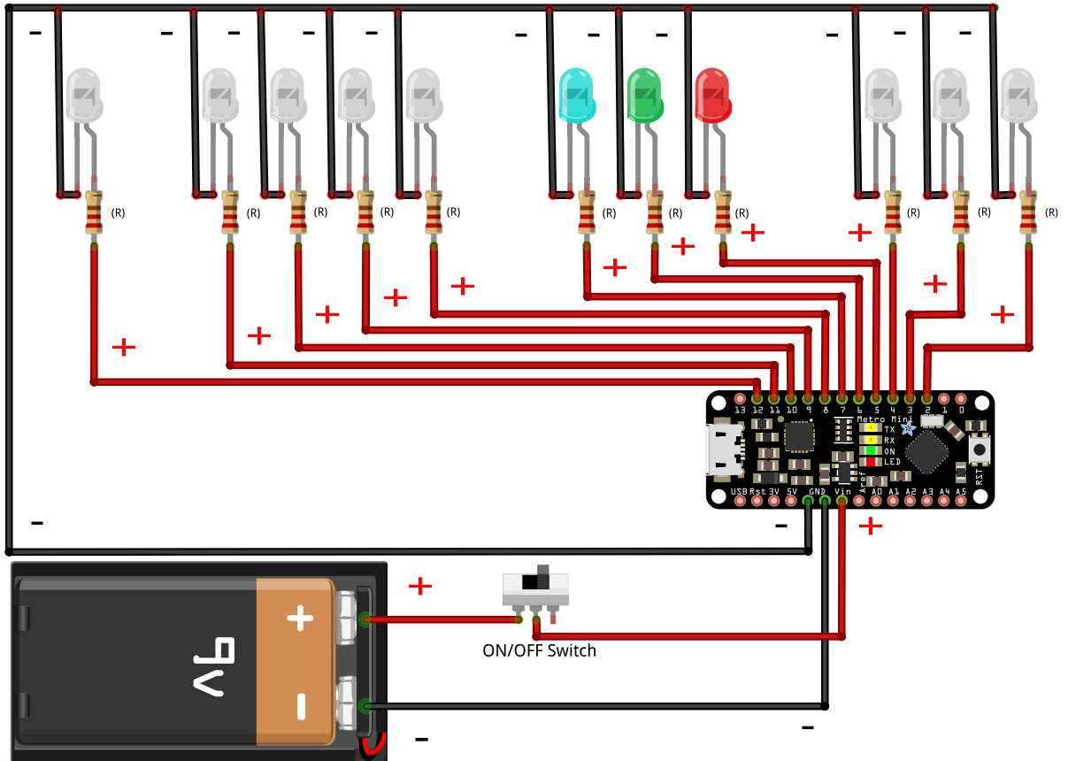
K-7 SPACE STATION WIRING DIAGRAM 2023
